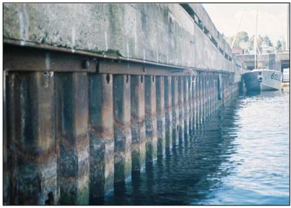
Existing steel sheetpile seawall between Central and West piers
